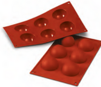
SF003 Half Sphere Size: Ø 60 h 30 mm Volume: 60 ml
